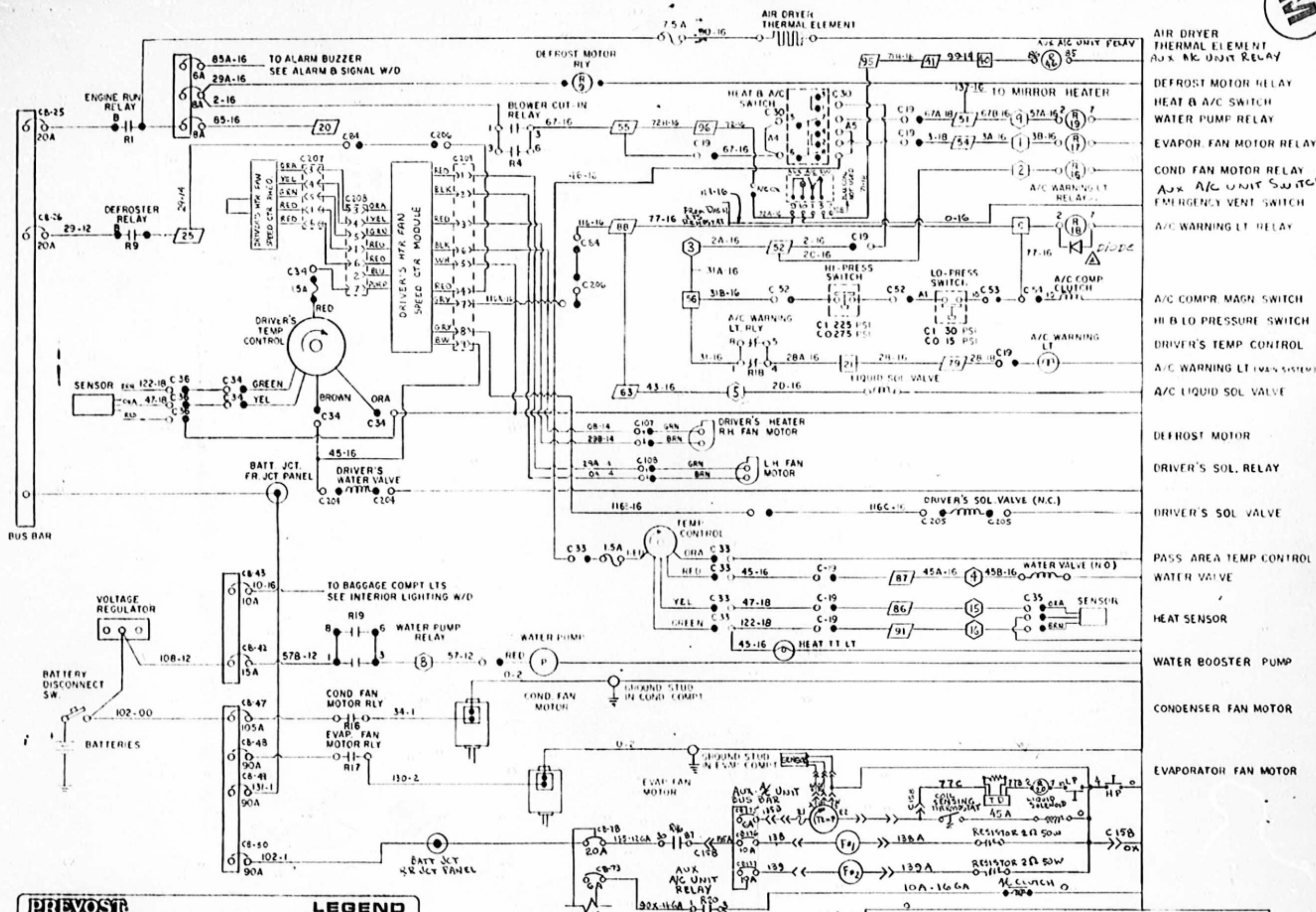
AIR CONDITIONING WIRING DIAGRAM WITH A/C AUXILIARY COACHES 102 EFF. W/L-545 PRIOR TO L-706 DATE: 87-07
